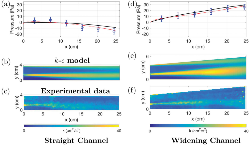
Figure 5. Comparison of k - \epsilon , simple model and experimental data, continued from Figure 4. In (a and d) streamwise pressure profiles are shown, with blue data points representing experimental data and red and black lines representing calculations from the k - \epsilon model and the simplified model, respectively. Error margins correspond to an accuracy of 0.5 mm in human eye measurements. In (b, c, e, f) time-averaged turbulent kinetic energy k is shown, calculated using the k - \epsilon model and PIV measurements.
